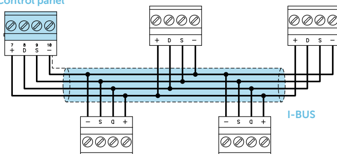
Control panel
